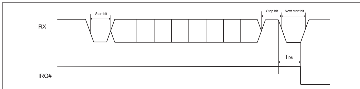
Figure 23. Receive Interrupt
