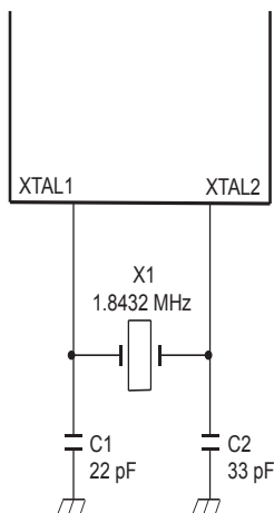
Figure 8. Crystal Oscillator Circuit Reference
