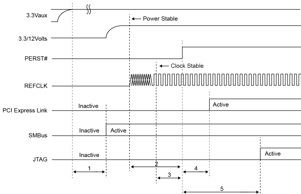
Figure 16-3 Initial Power-up
