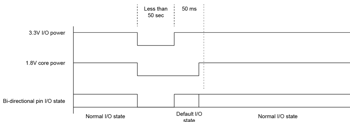
Figure 16-2 Recommended Power Sequence
