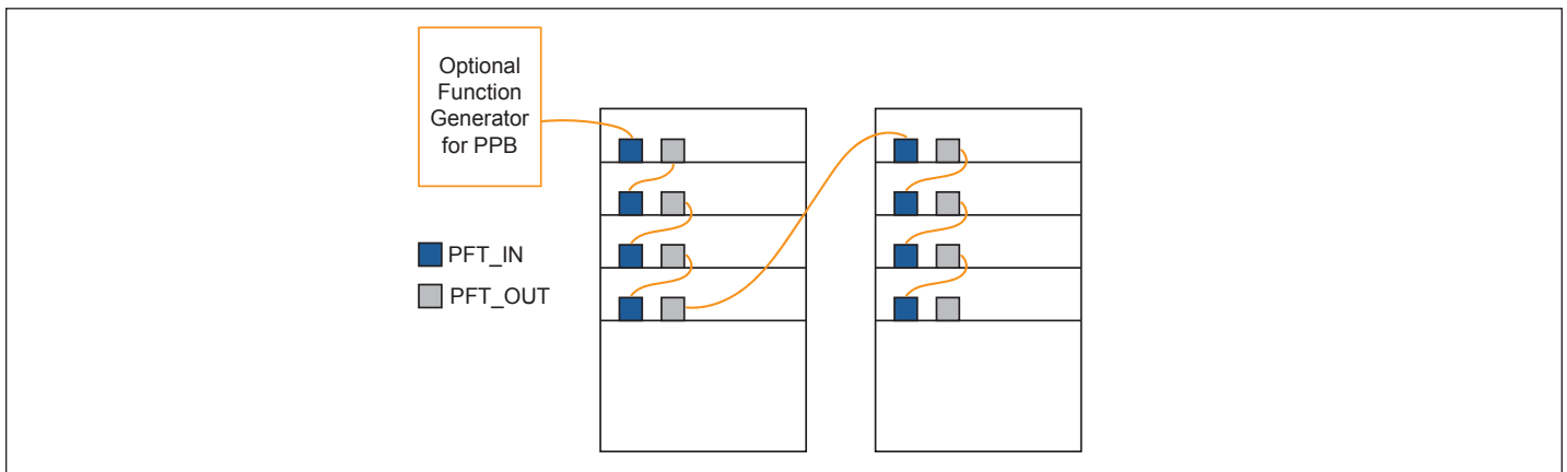
Figure 9. Frequency Lock
