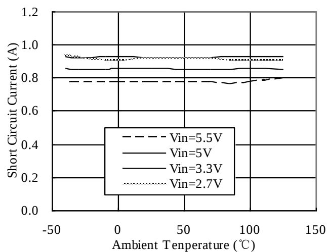
Short-Circuit Output Current vs. Ambient Temperature
