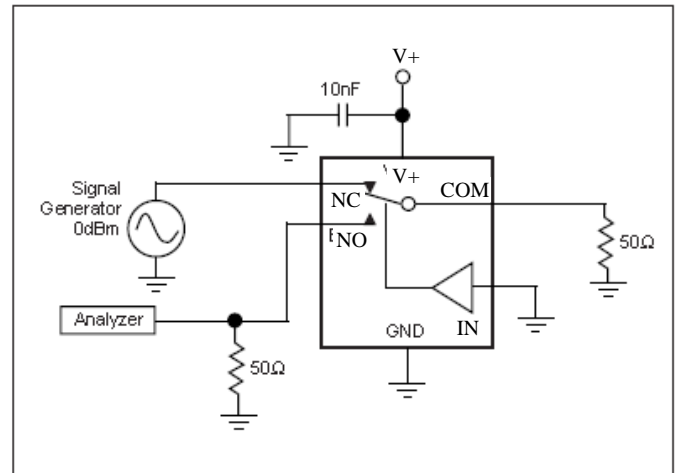
Figure 5. Crosstalk
