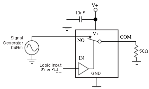
Figure 8. Bandwidth
