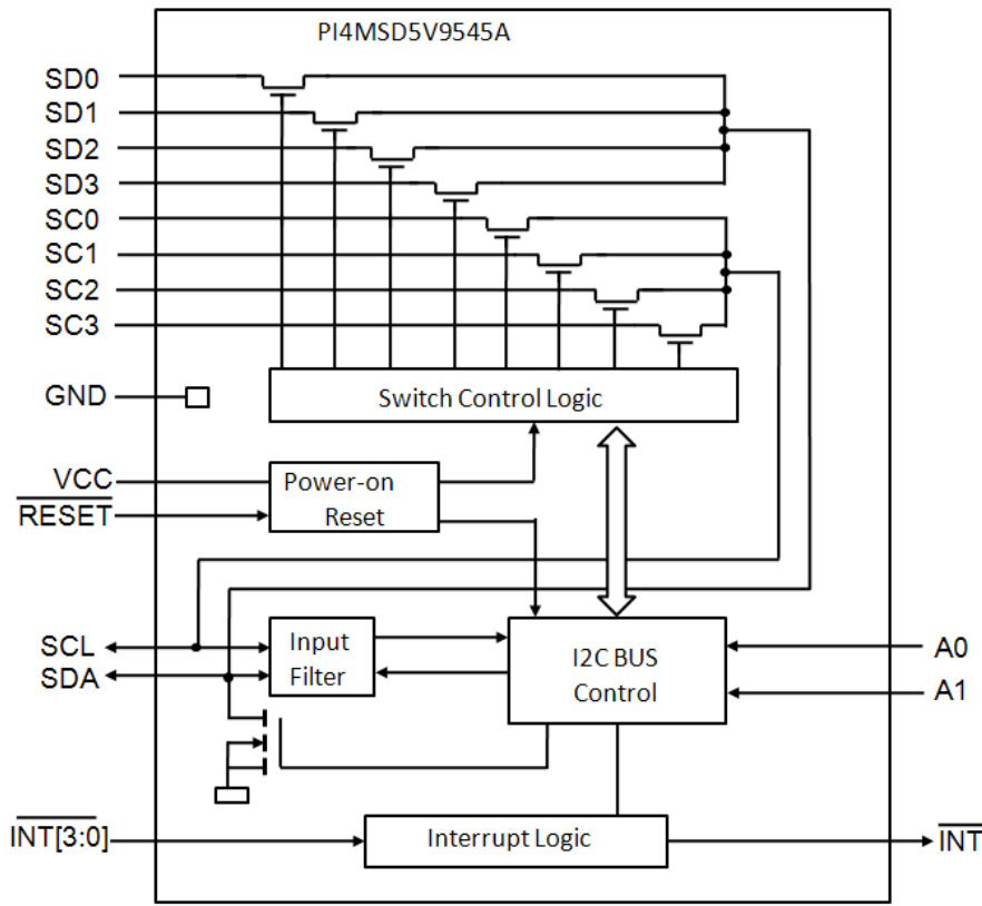
Figure 1: Block Diagram
