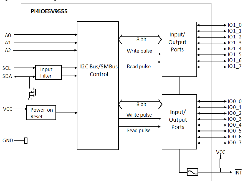
Figure 4: Block diagram
