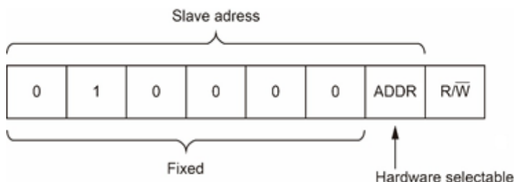
Fig. 10: PI4IOE5V6416 address
