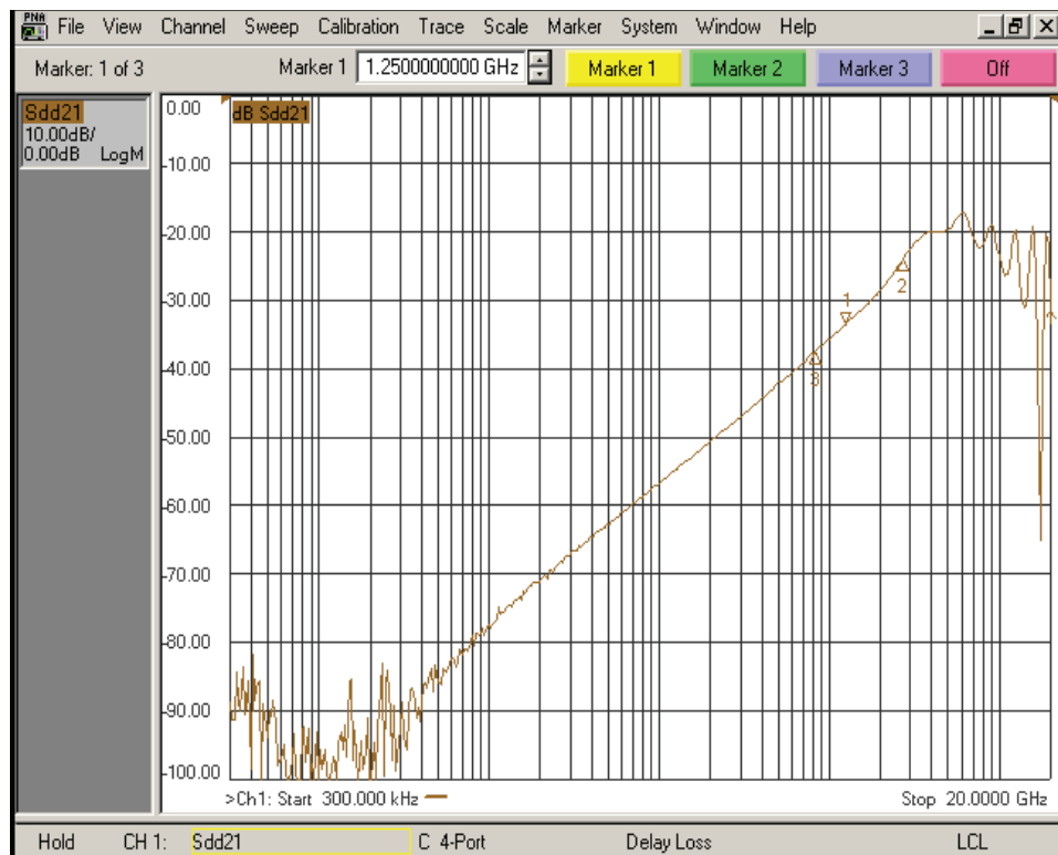
Fig 5. Off Isolation
