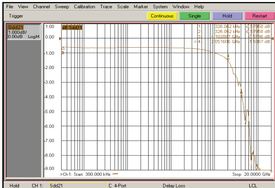
Fig 6. Insertion Loss
