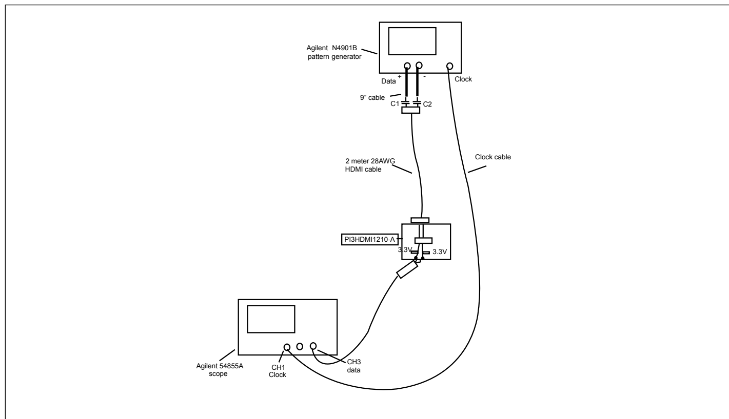
Figure 7. TMDs TP3 Rx "switch at receiver" eye compliance test setup
