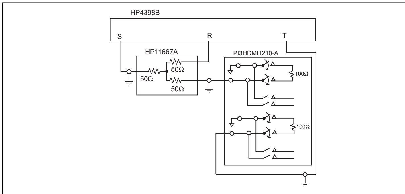
Fig 1. Crosstalk Setup
