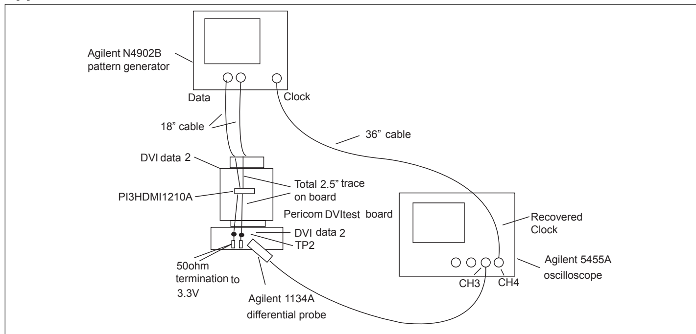
Figure 6. TMDs TP2 Tx eye compliance test setup
