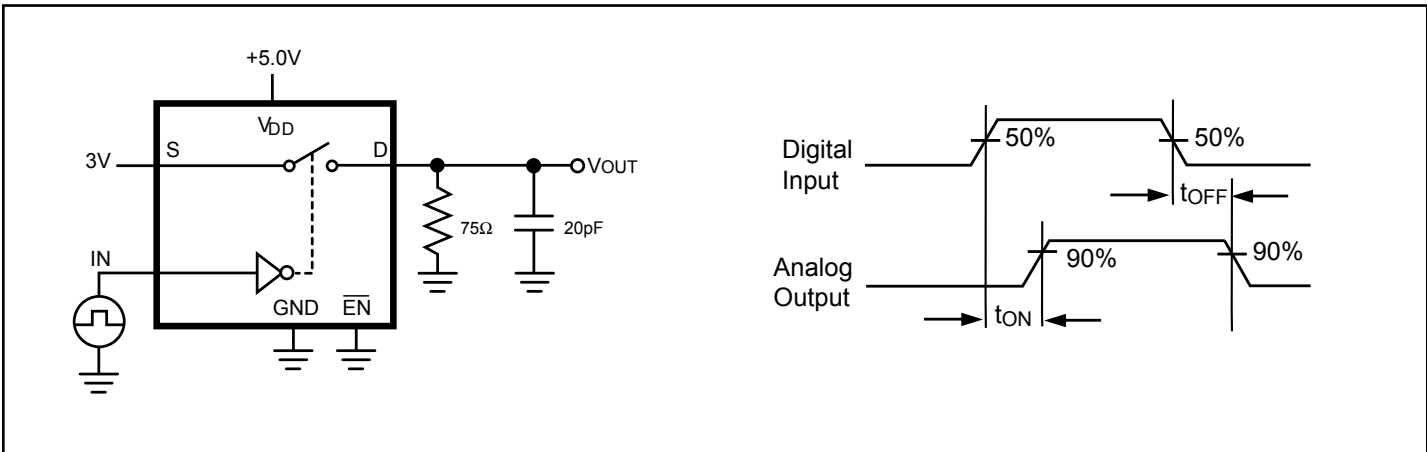
Figure 4. Switching Time
