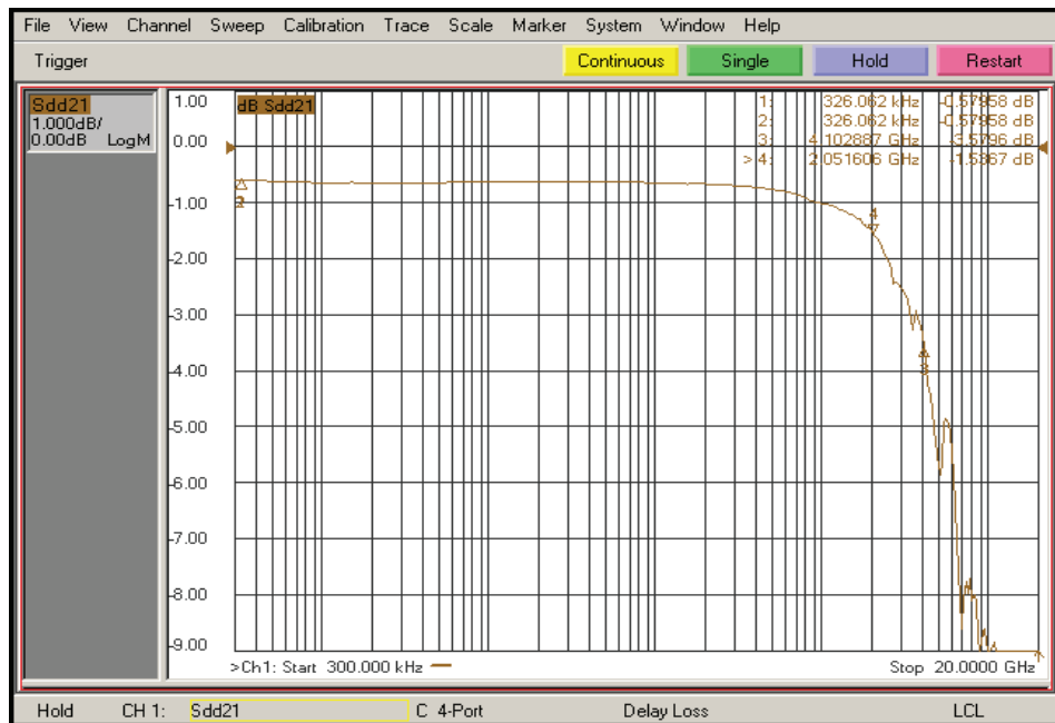
Fig 6. Insertion Loss
