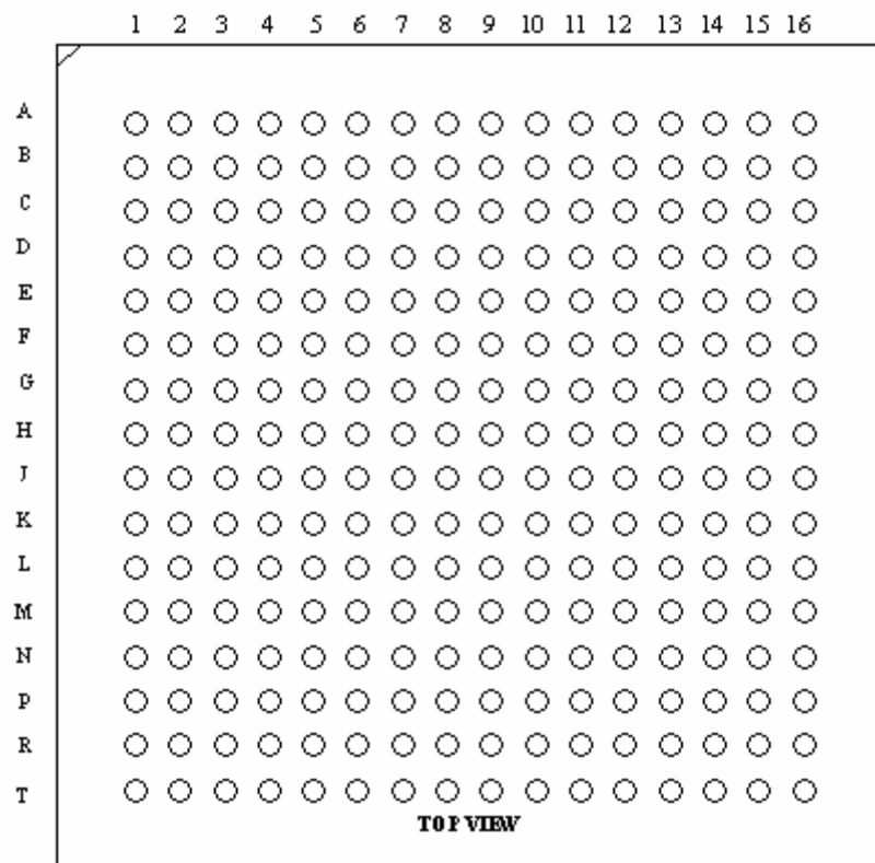
Figure 17-19 Top View Drawing
