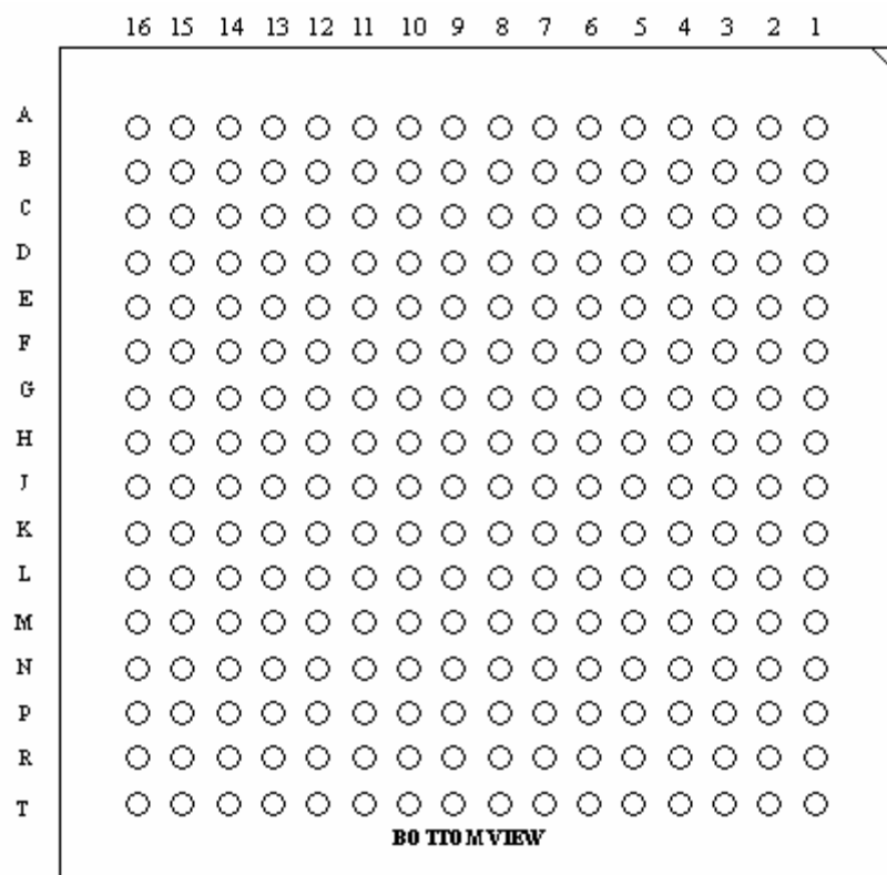
Figure 17-20 Bottom View Drawing
