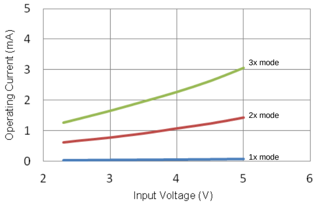
Operating Current vs Input Voltage (No Load)
