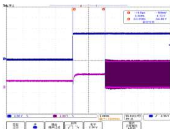
Startup Response
