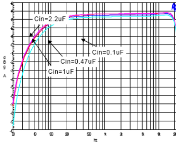
7. Frequency Response
