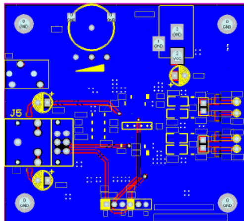
Figure 3. Bottom Layer
