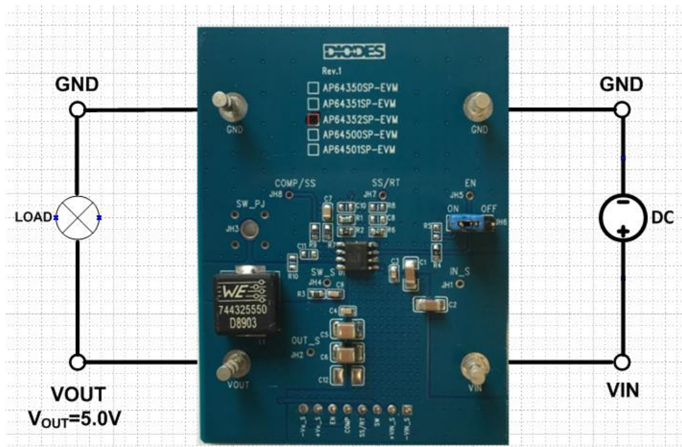
Figure 2. AP64352SP-EVM
