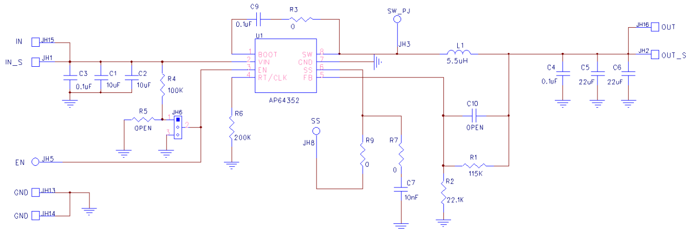
Figure 3. AP64352SP-EVM Schematic
