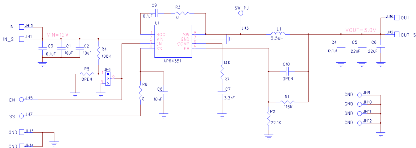
Figure 3. AP64351SP-EVM Schematic
