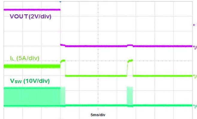
Figure 9. Output Short Protection, IOU=3.5A
