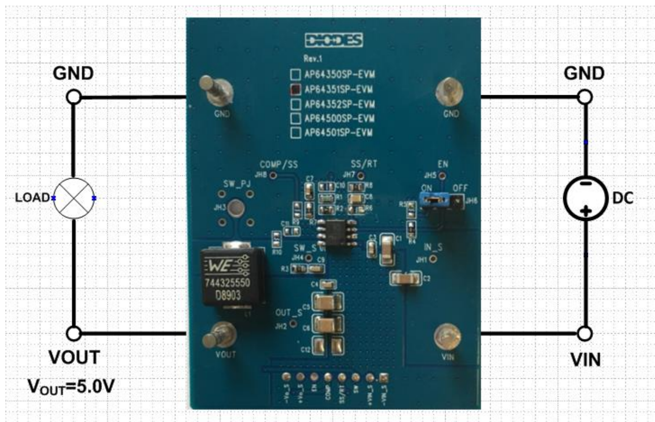
Figure 2. AP64351SP-EVM
