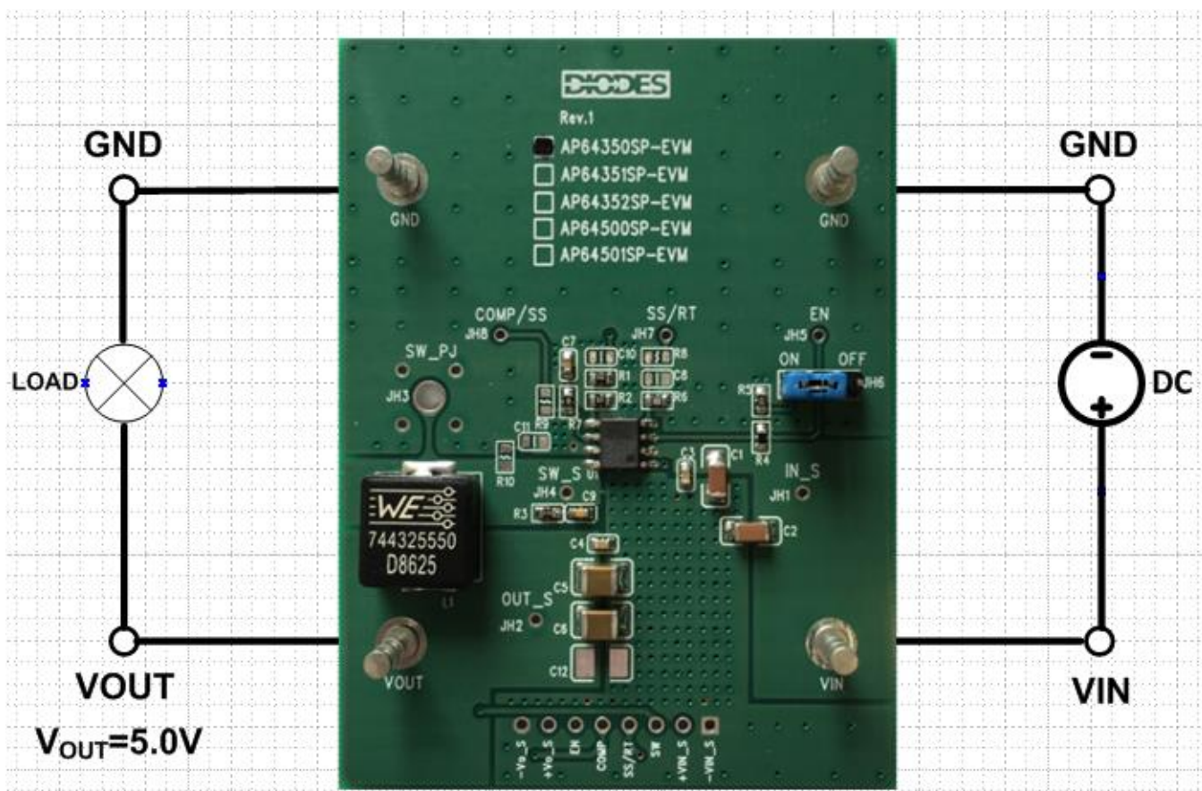
Figure 2. AP64350SP-EVM
