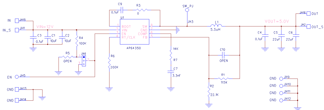
Figure 3. AP64350SP-EVM Schematic
