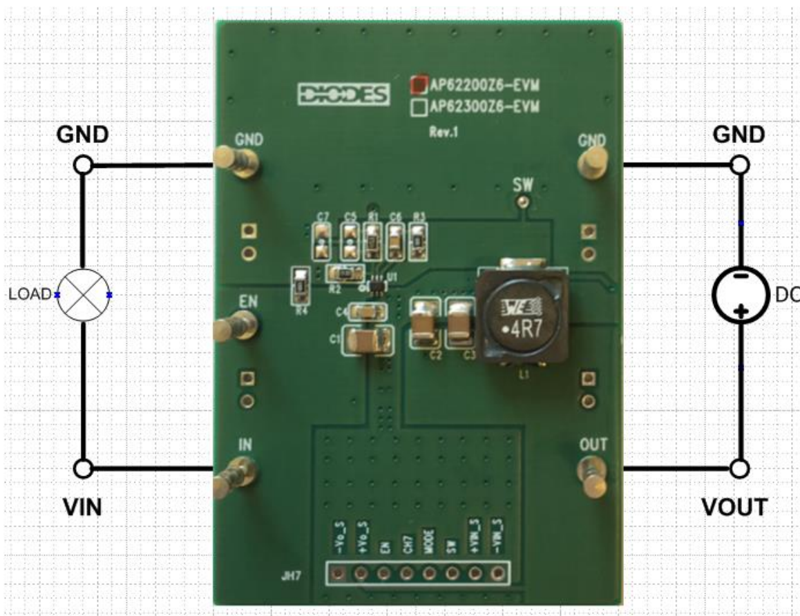
Figure 2. AP62200Z6-EVM
