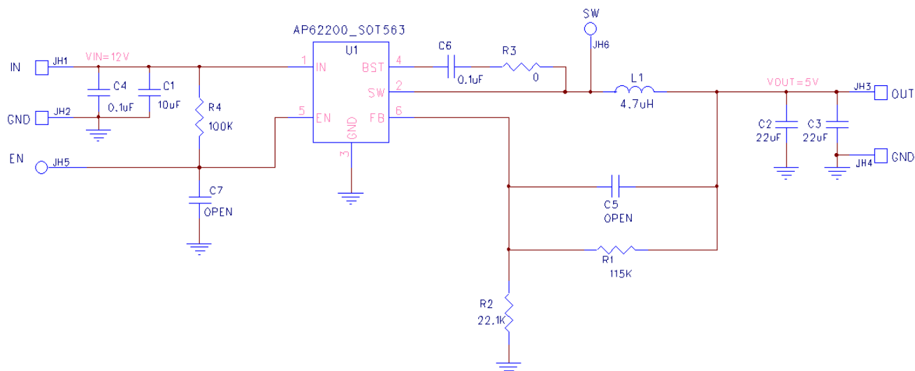
Figure 3. AP62200Z6-EVM Schematic
