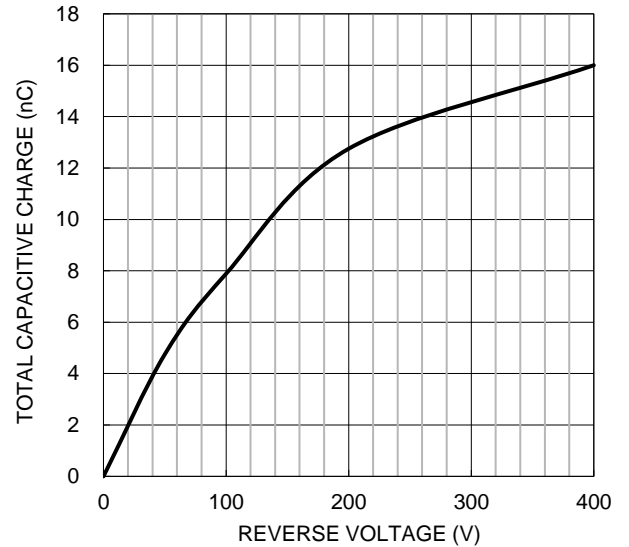
Figure 6. Typical Capacitive Charges
