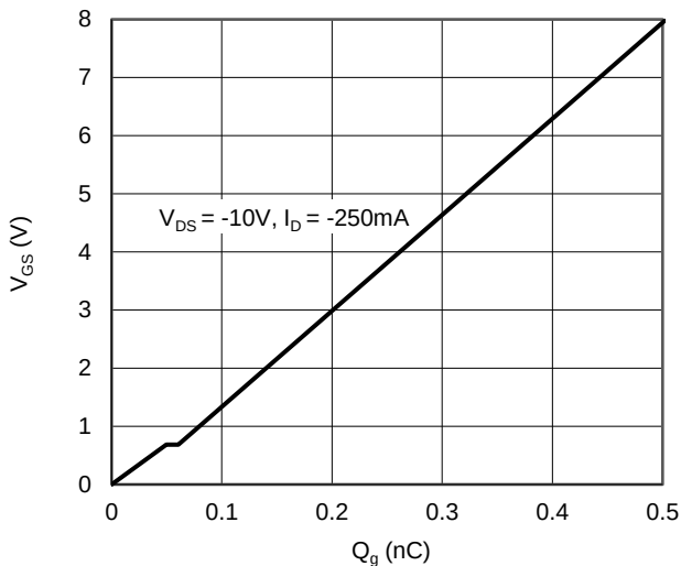
Figure 11. Gate Charge
