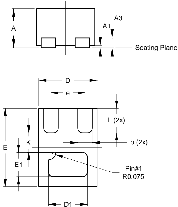
X2-DFN0806-3
