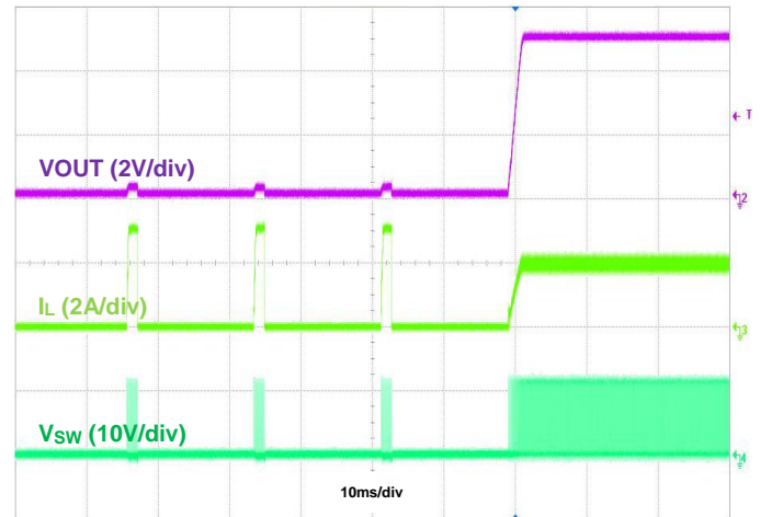
Figure 24. Output Short Recovery, I_{OUT} = 2\text{A}
