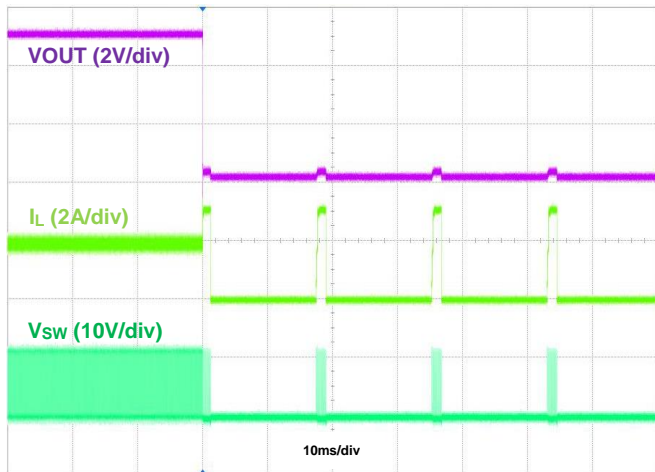
Figure 23. Output Short Protection, I_{OUT} = 2\text{A}
