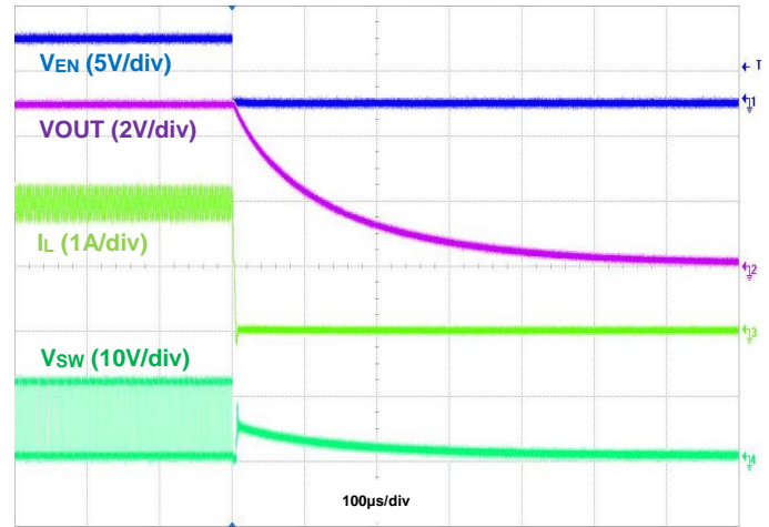
Figure 22. Shutdown Using EN, I_{OUT} = 2\text{A}
