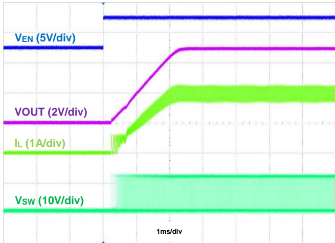
Figure 21. Startup Using EN, I_{OUT} = 2\text{A}
