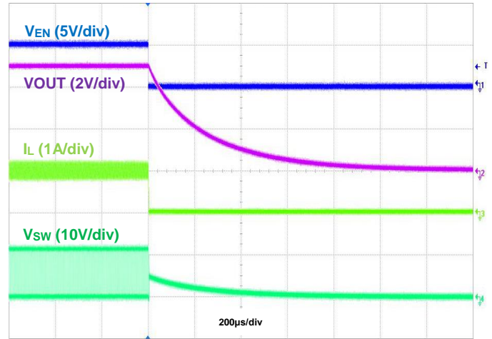
Figure 22. Shutdown Using EN, I_{OUT} = 1\text{A}
