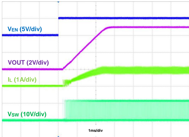
Figure 21. Startup Using EN, I_{OUT} = 1\text{A}
