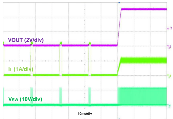
Figure 24. Output Short Recovery, I_{OUT} = 1\text{A}
