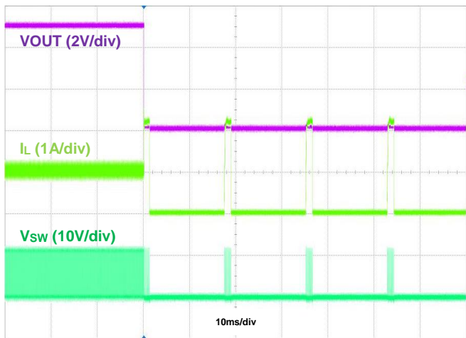
Figure 23. Output Short Protection, I_{OUT} = 1\text{A}
