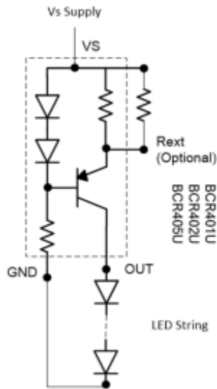
Figure 1. Typical Application Circuit for BCR40X LED Driver
