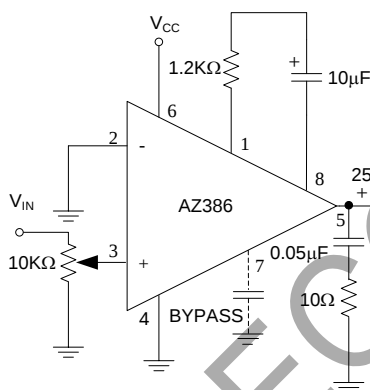
Amplifier With Gain=50
