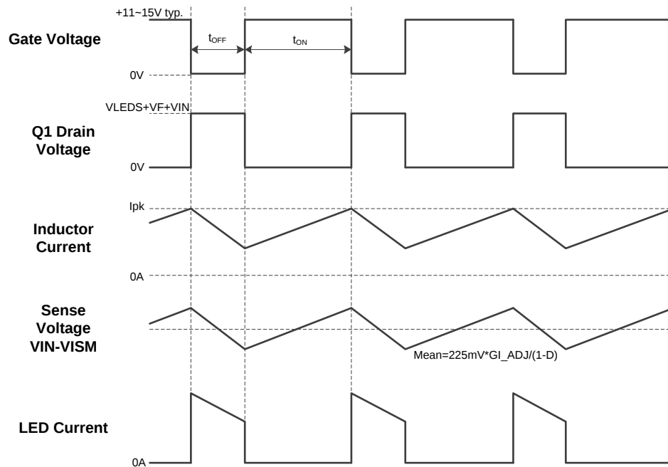
Figure 3. Operating Waveforms
