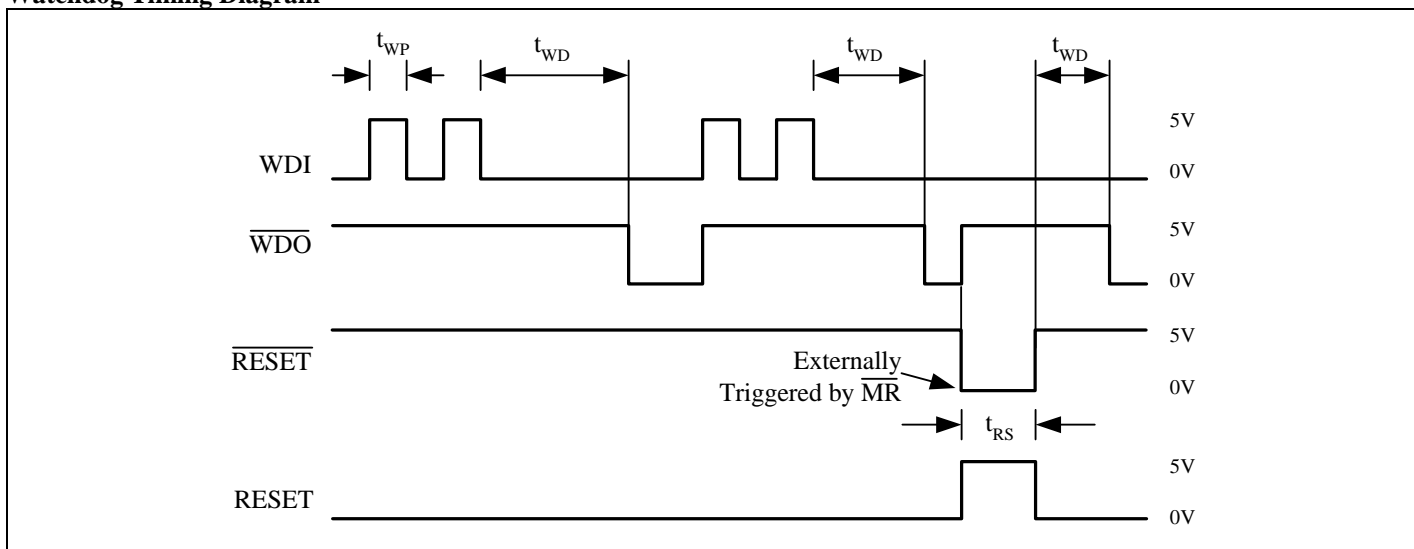
Watchdog Timing Diagram
