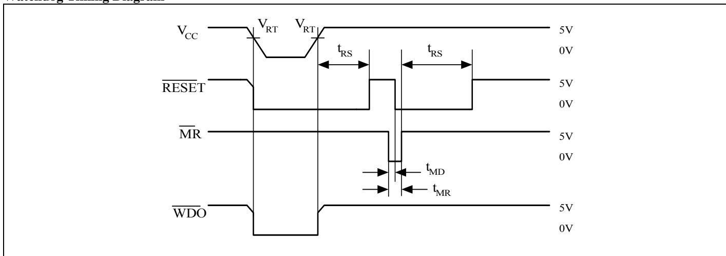
Watchdog Timing Diagram
