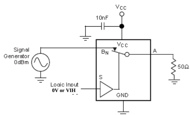
Figure 9. Bandwidth
