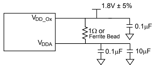
Figure 3. Power Supply Filter
