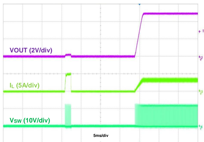
Figure 22. Output Short Recovery, IOUT = 3.5A
