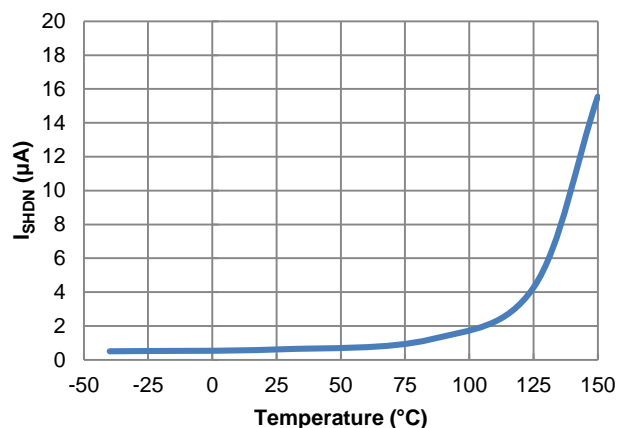
Figure 11. I_{SHDN} vs. Temperature
