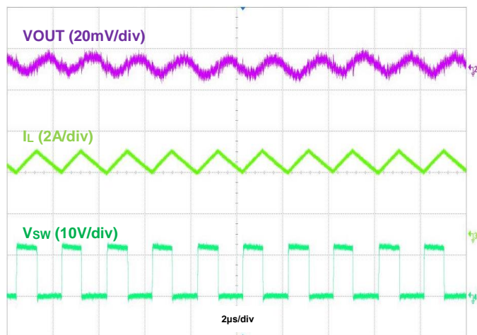
Figure 15. Output Voltage Ripple, I_{OUT} = 3.5\text{A}
