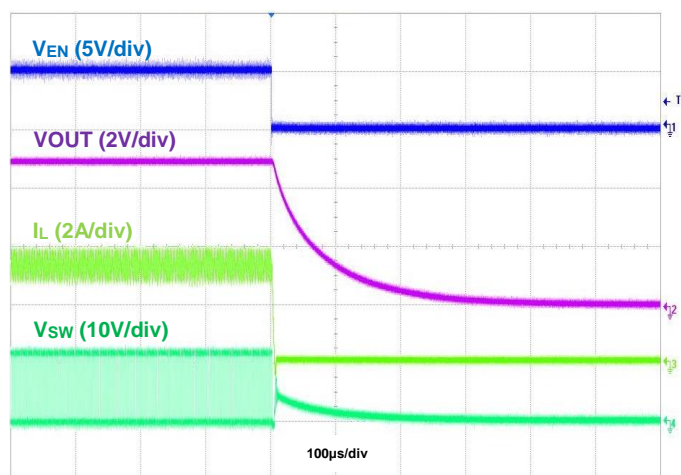
Figure 20. Shutdown Using EN, IOUT = 3.5A
