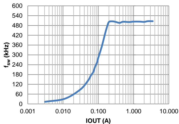
Figure 13. f_{sw} vs. Load
