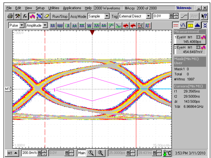
Output Eye
