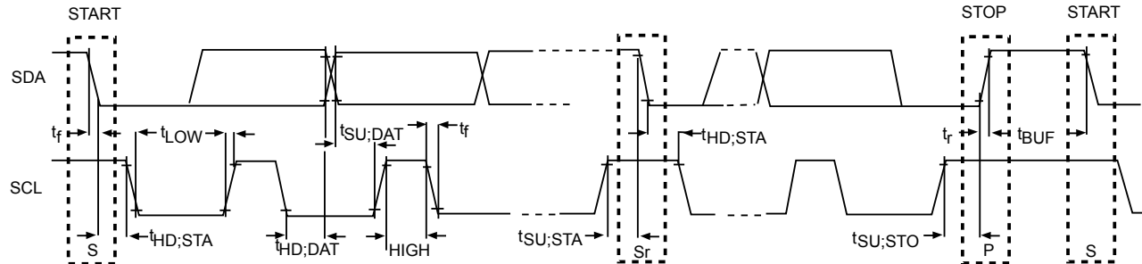
I²C Timing
