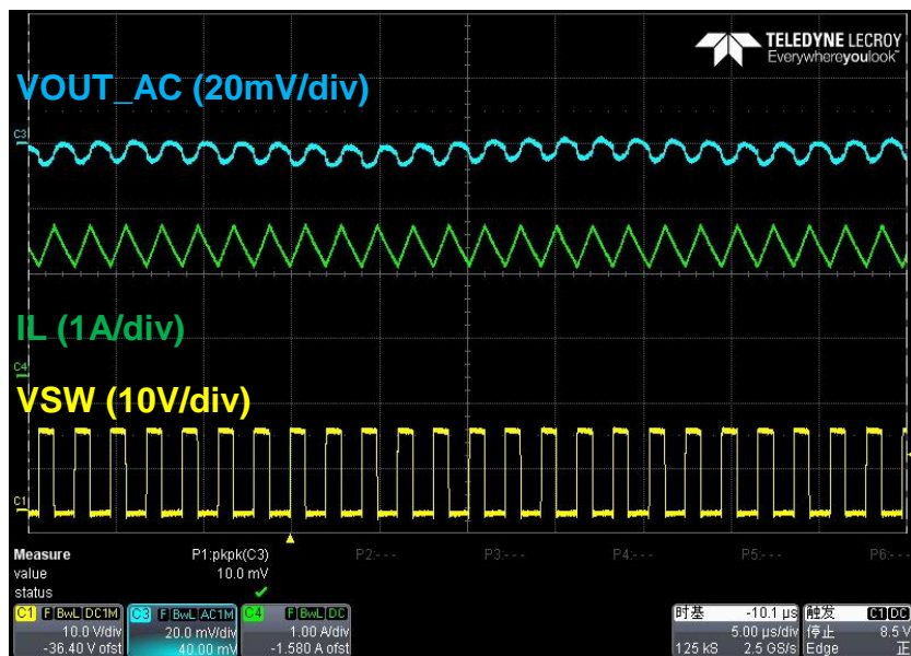
Figure 5. Output Ripple for VIN=12V, VOUT=3.3V, IOUT=2A
