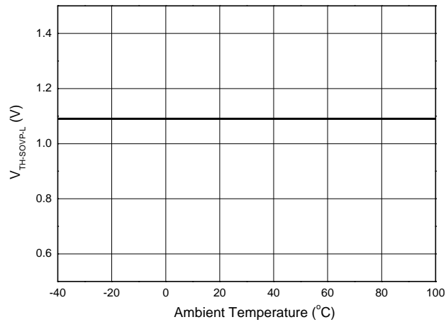
V_{TH-SOVP-L} vs. Ambient Temperature
