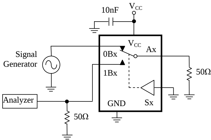
Figure 5. Crosstalk
