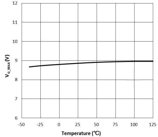
Figure 4. Maximum Gate Voltage vs. T_A
