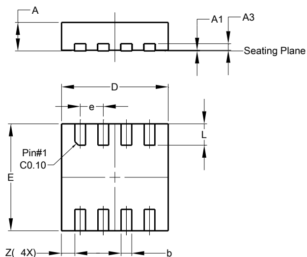
V-DFN3030-8
