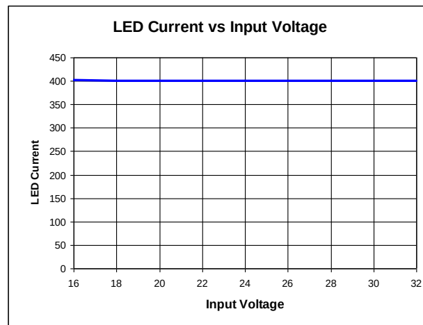
Figure 45 Line Regulation
