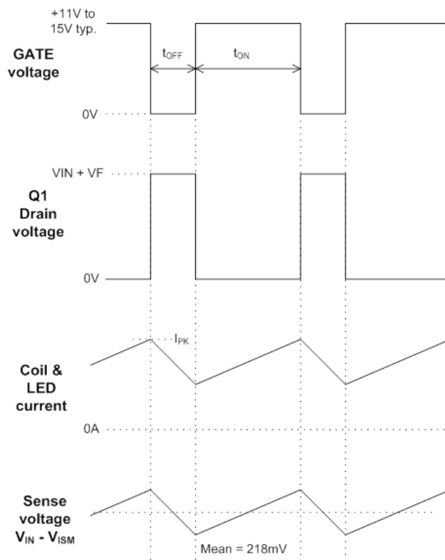
Figure 21 Buck Configuration
