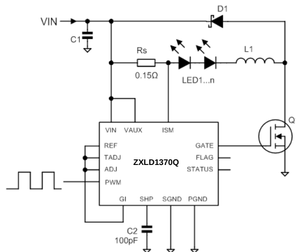
Figure 21 Buck Configuration
