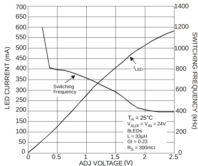
Figure 6 Buck-Boost LED Current, Switching Frequency vs. V_{ADJ}
