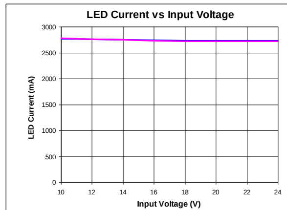
Figure 42 Line Regulation
