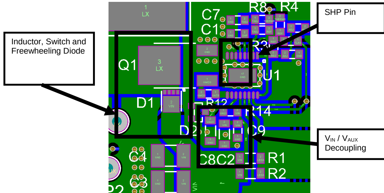
Figure 39 Circuit Layout
