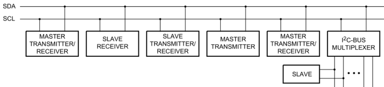
Figure 9. System Configuration
