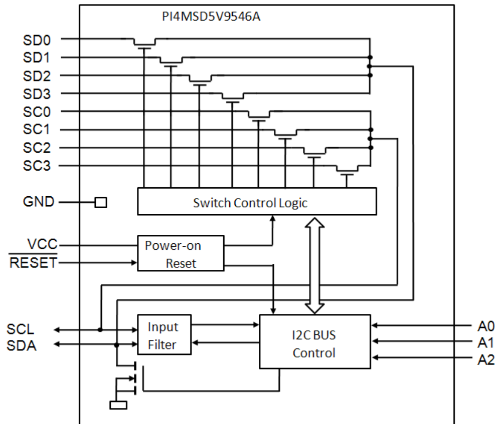
Figure 1: Block Diagram
