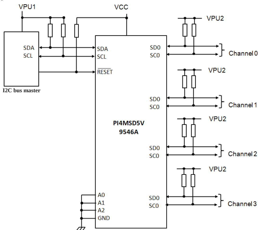
Figure 3. Typical Application
