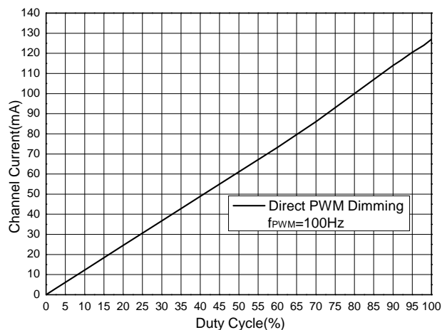
Direct PWM Dimming @ f_{\text{PWM}}=100\text{Hz} Channel Current vs. Duty Cycle
