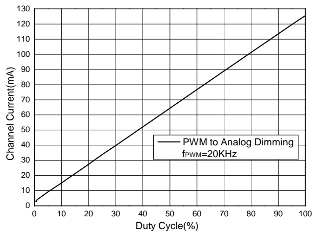
PWM to Analog Dimming @ f_{\text{PWM}}=20\text{kHz} Channel Current vs. Duty Cycle
