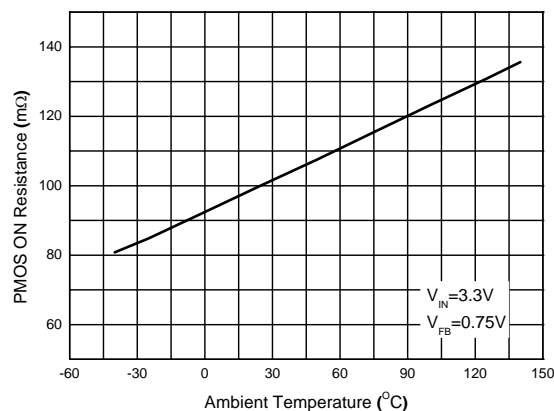
PMOS ON Resistance vs. Ambient Temperature
