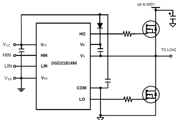
Typical Configuration
