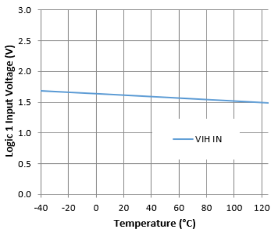
Figure 17. Logic 1 Input Voltage vs. Temperature
