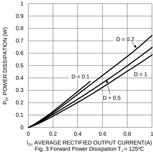
Fig. 3 Forward Power Dissipation T_J = 125^\circ\text{C}
