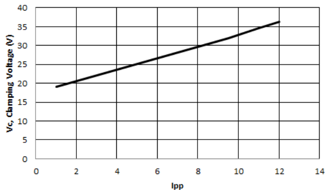
Figure 7, Clamping Voltage Characteristic (tp=8/20μs)
