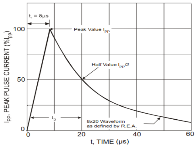
Figure 3, typical 8 x 20μs pulse waveform
