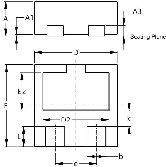
X2-DFN1010-3
